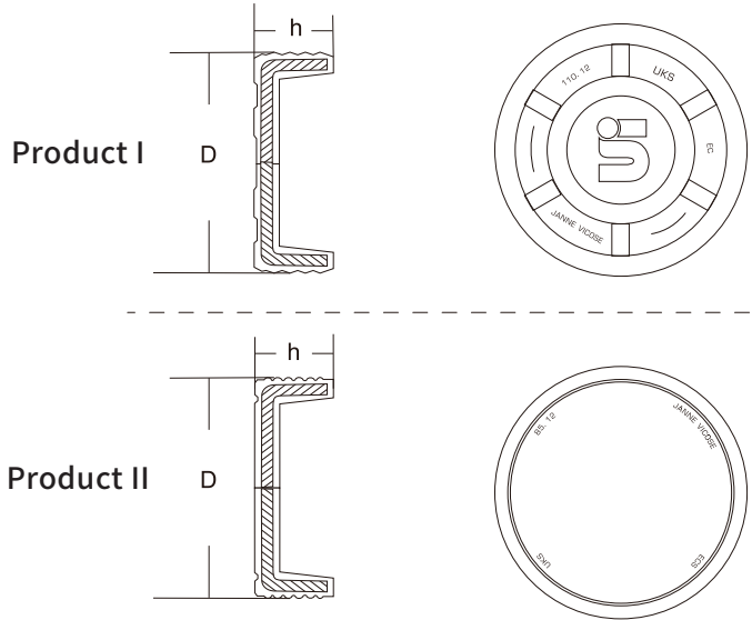
Cross section
